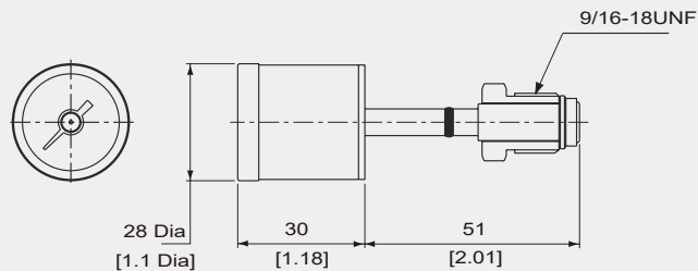
Male Swivel
