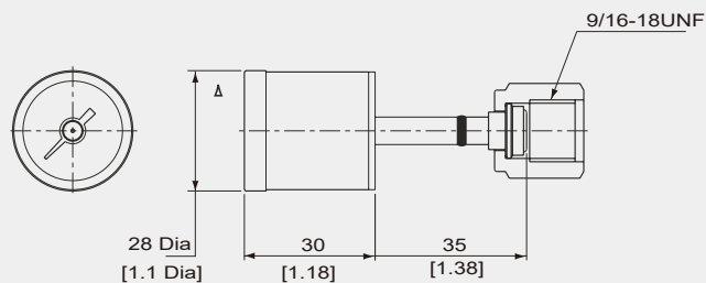
Female Swivel
